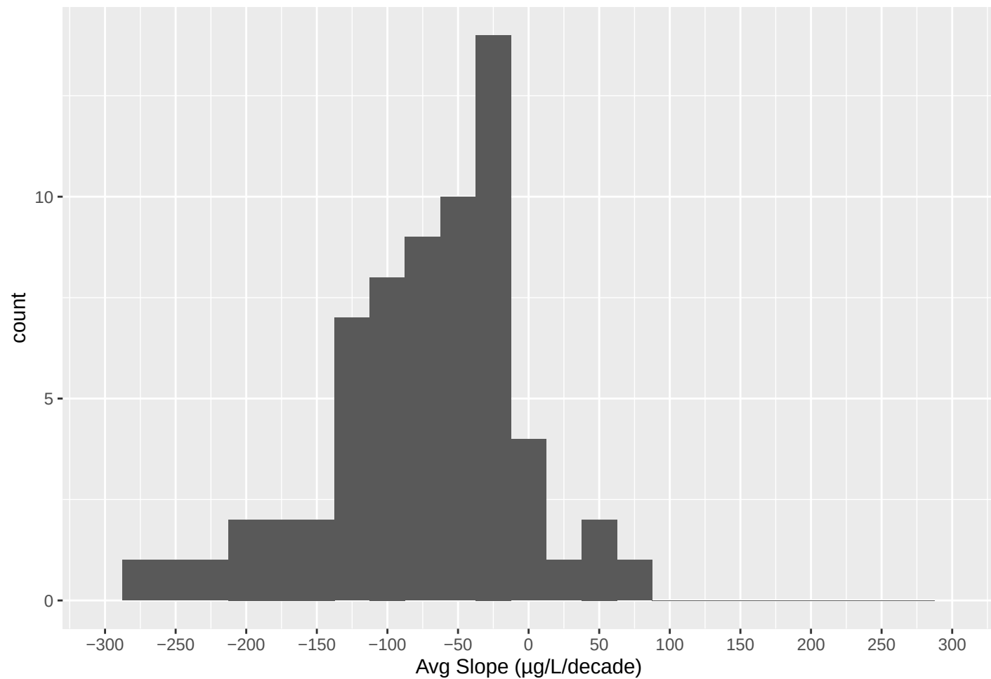
NO 2 /3 Slope Distribution Histogram, Zoomed-in, bin-width = 25
